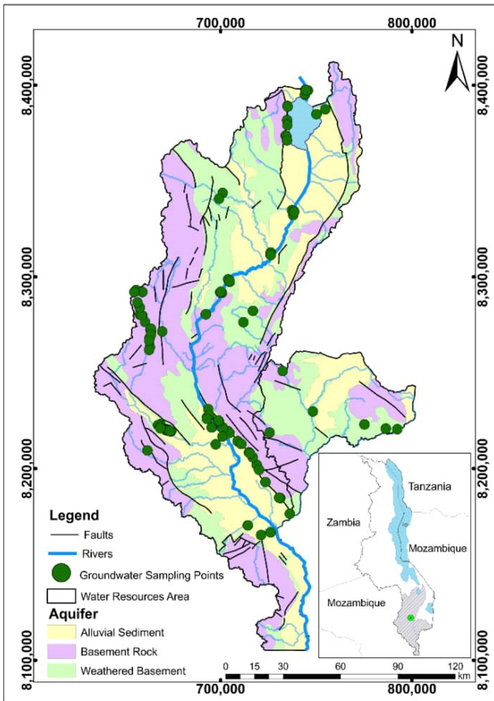
Figure 2. Study area showing aquifer types and survey groundwater-sampling points.
