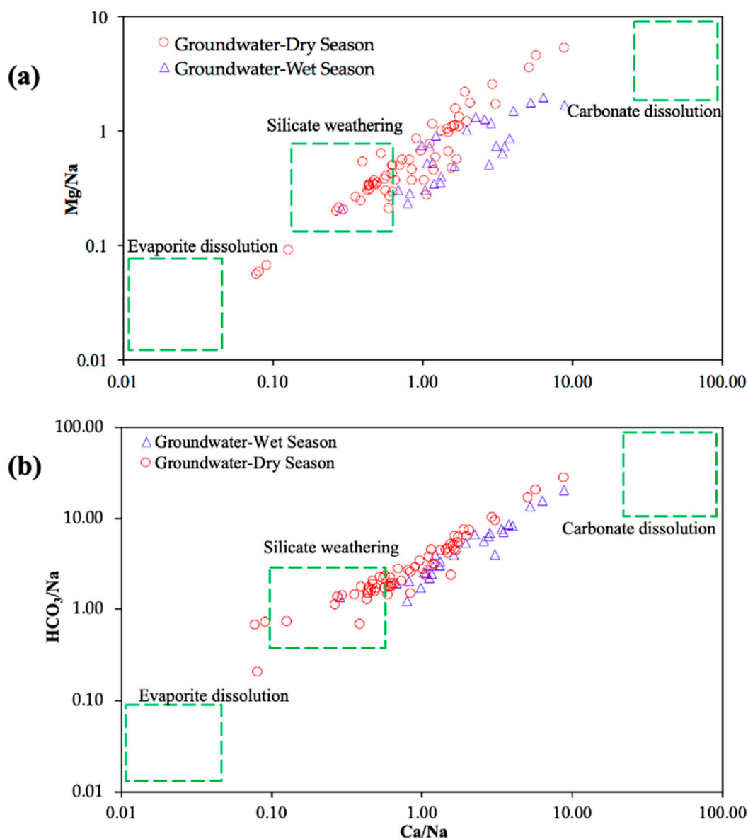
Figure 11. Bivariate plots of molar ratios. (a) Na-normalised Mg vs. Na-normalised Ca and (b) Na-normalised HCO 3 vs. Na-normalised Ca.
